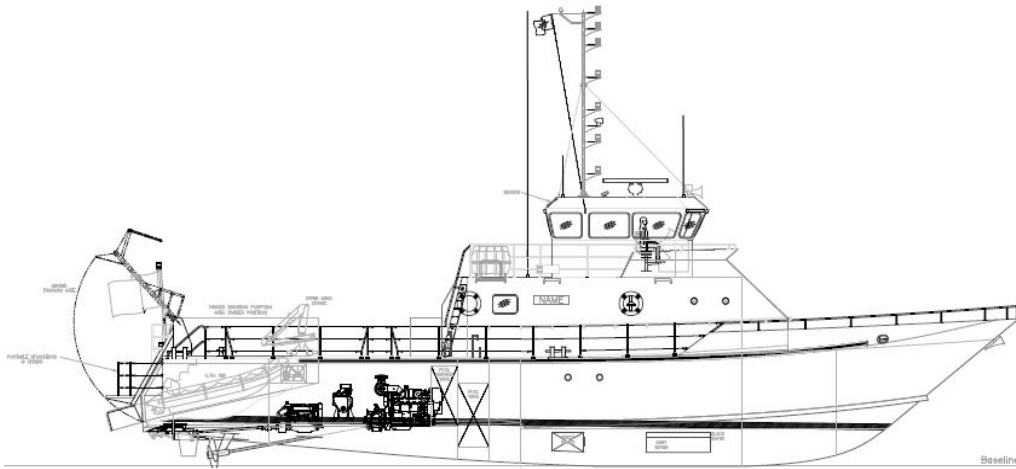
SIDE VIEW
