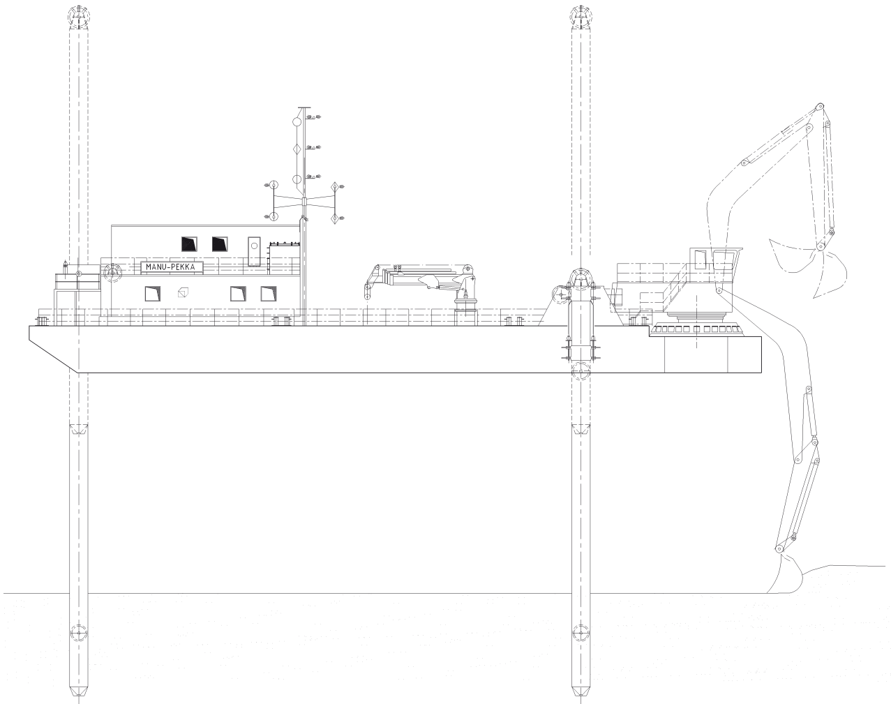
SIDE VIEW
